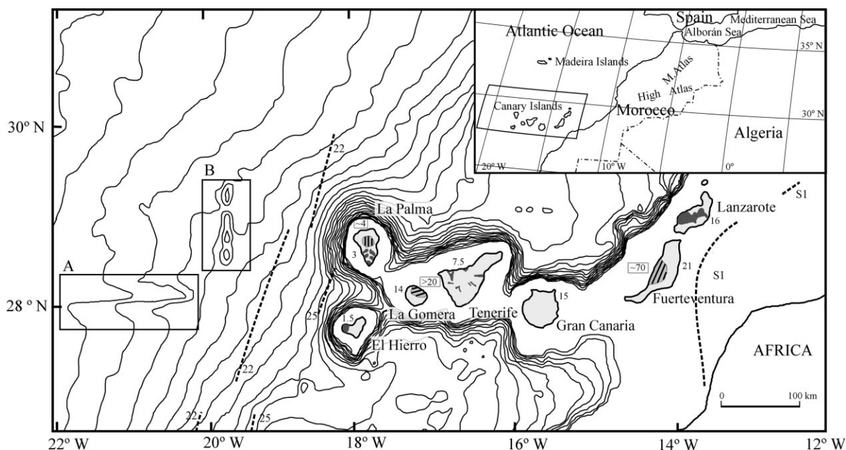
Fig. 1. A map of the Canary Islands showing some bathymetric (contours at 100 m intervals but only at depths greater than 2.5 km), chronological, and eruptive activity data. In dark grey, terrain covered by historical eruptions. Striped, basal complexes (stripe directions in the azimuth of the sheeted dike complex). Numbers indicate the ages (Ma) of the oldest subaerial outcrops; when in boxes, the ages of the basal complexes. Boxes A and B underline tectonic signatures: A is a straight, 300 km-long submarine canyon, and the site of a M = 6.2 quake which happened in 1959. B is a 200 km-long seamount line parallel to the strike of the sheeted dike complex of La Palma, the nearest island.
