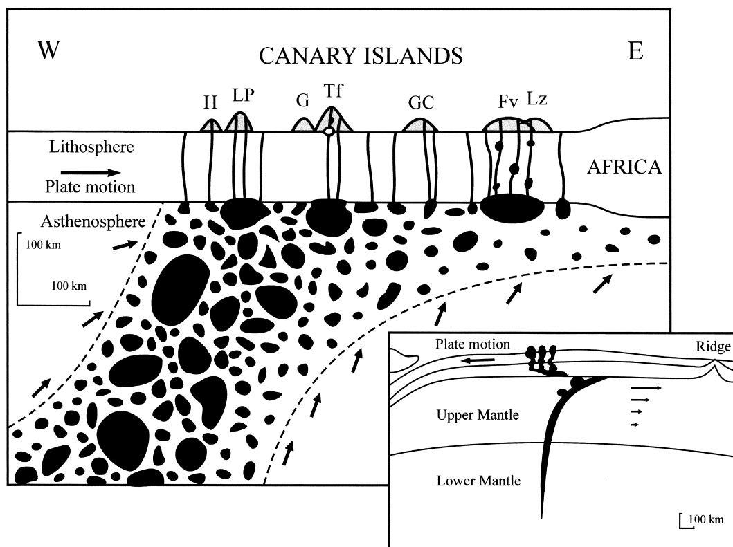
Fig. 3. The blob model for the Canary Islands, after Hoernle and Schmincke (1993). Inset: dipping plume model for the Hawaiian Islands after Ihinger (1995). Note that, due to upper mantle flow towards the spreading ridge (and contrary to the Canary model), the conduit dips against the lithosphere plate motion. See text for a different model (Cox, 1999).
