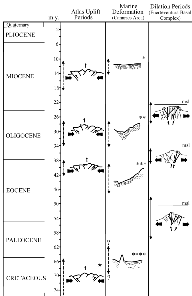
Fig. 9. A calendar of tectonic and magmatic events in the Atlas chain, the Canary Islands and the intervening Atlantic Ocean. Atlas uplift periods as cited in Uchupi et al. (1976), excepting (*) after Froitzheim et al. (1988). Marine deformations in the Canary area after: (*) McMaster and Lachance (1968); (**) Uchupi et al. (1976); (***) Summerhayes et al. (1971); (****) Dañobeitia and Collette (1989). The first three are coincident in time with erosional unconformities described by Hinz et al. (1982). Dilation periods in the Fuerteventura basal complex after Stillman (1987). Though based on real sections, sketches are only approximate renderings.
