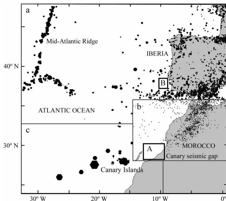
Fig. 10. Recent seismicity in the Canary Islands and surrounding areas. Since no author plots the African and Atlantic foci together, different sources have been used: (a) is from Andeweg et al. (1999); (b) from Medina and Cherkaoui (1991); and (c) from Wyssession et al. (1995). Boxes indicate (A) the Canary Islands, and (B) the Lisbon seismic gaps. Both are proposed to be due to the unusual mass of sediments deposited on the continental slope and rise. In (a) and (c), the size of the signs correlates with seismic magnitude.
