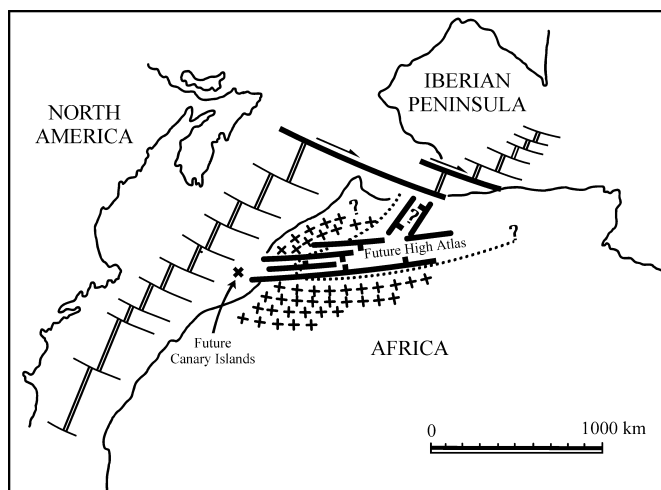
Fig. 5. The ultimate cause for the origin of the Canary Islands may well be the formation in Jurassic times of this failed arm rift in the place of the present High Atlas, during the opening of the central Atlantic Ocean. Redrawn from Lee and Burgess (1978).
