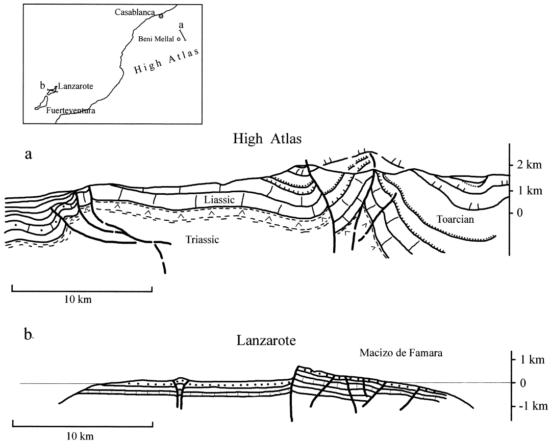
Fig. 6. (a) A flower structure cropping out in the High Atlas (after Laville and Piqué, 1992). (b) An E–W section (along the parallel 29°N) across Lanzarote, an island of medium size, at the same horizontal and vertical ( 2\times ) scales. The tectonic structures are from Marinoni and Pasquaré (1994).
