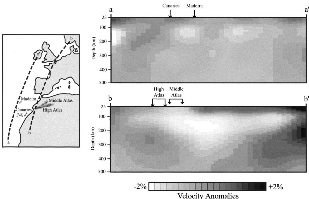
Fig. 4. Results of the seismic tomography experiment performed by Hoernle et al. and which are pertinent for the origin of the Canary Islands. In the a-a' section a cold lithosphere can be seen underlying the Canary Islands; the islands, moreover, overlie the border of a mild thermal anomaly of the upper mantle. In the b-b' section, a much more important thermal anomaly is located under the Atlas Mountains. Redrawn from Hoernle et al. (1995).
