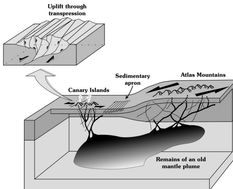
Fig. 8. Cartoon illustrating the unifying hypothesis on the origin of the Canary Islands. The inset represents a transpressive phase, when the islands would emerge as flower structures.
