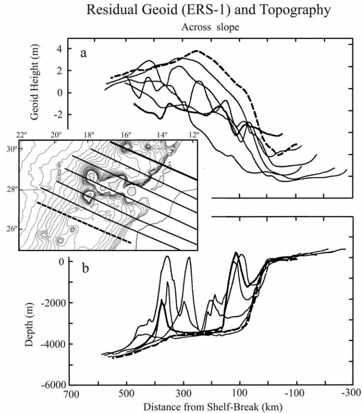
Fig. 2. Geoid height (a) and topography (b) around the Canary Islands. Note that the thicker and dashed lines correspond in both cases to the northernmost and southernmost sections. All geoid heights in the islands area are lower than the geoid at the southernmost section, far from the islands. As for the bathymetric baselines, they are almost identical among the islands and outside them (dashed line). After Watts (1994).
